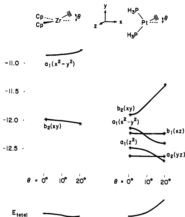
Figure 5. Walsh diagram for moving the acetylene off the symmetry axis, for Cp 2 Zr(acetylene) [left] and Pt(PH 3 ) 2 (acetylene) [right]. Orbitals are labeled according to their symmetries in C 2v ( \theta = 0^\circ ) and their dominant d-orbital components.
