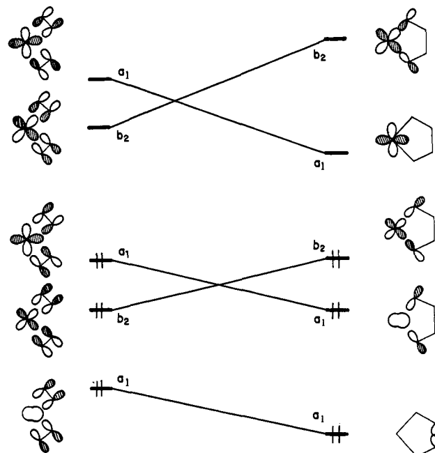
Figure 7. Schematic correlation diagram for coupling two acetylenes on Cp_2Zr . The highest filled orbitals of the bis(acetylene) compound (left) are derived from bonding combinations of the incoming acetylene \pi -orbital with orbital "B" of Figure 6 and the incoming acetylene \pi^* -orbital with orbital "D" of Figure 6. The out-of-plane acetylene \pi -orbitals correlate smoothly with metallacycle \pi -orbitals and are omitted for clarity.
